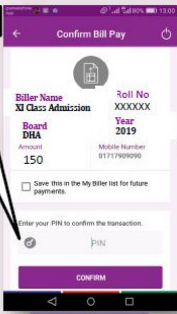
Step -6
